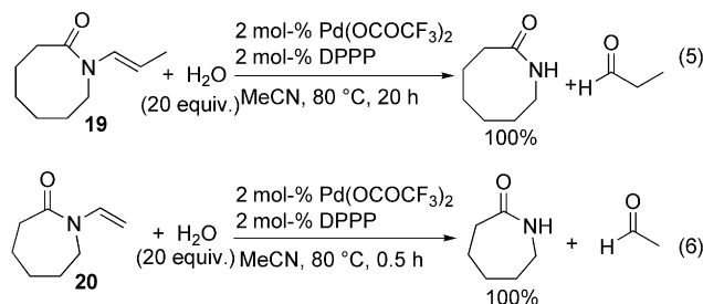
Scheme 5. Hydrolytic deallylation of N -1-propenyl and N -vinyl amide.
