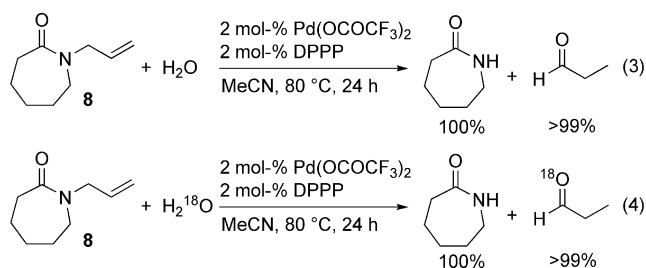
Scheme 4. Pd-catalyzed hydrolytic deallylation of 8 with 18 O-labeled water.
