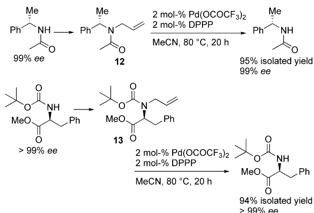
Scheme 1. Hydrolytic deallylation of optically active N -allyl amides.
