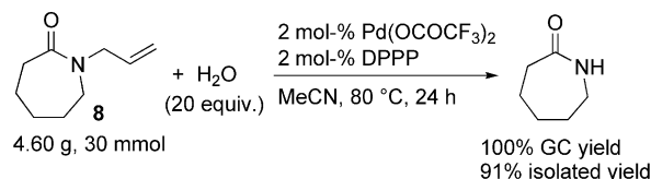
Scheme 2. Hydrolytic deallylation on 30 mmol scale.
