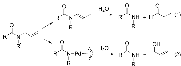
Scheme 3. Possible pathways of Pd-catalyzed hydrolytic deallylation of N -allyl amides.
